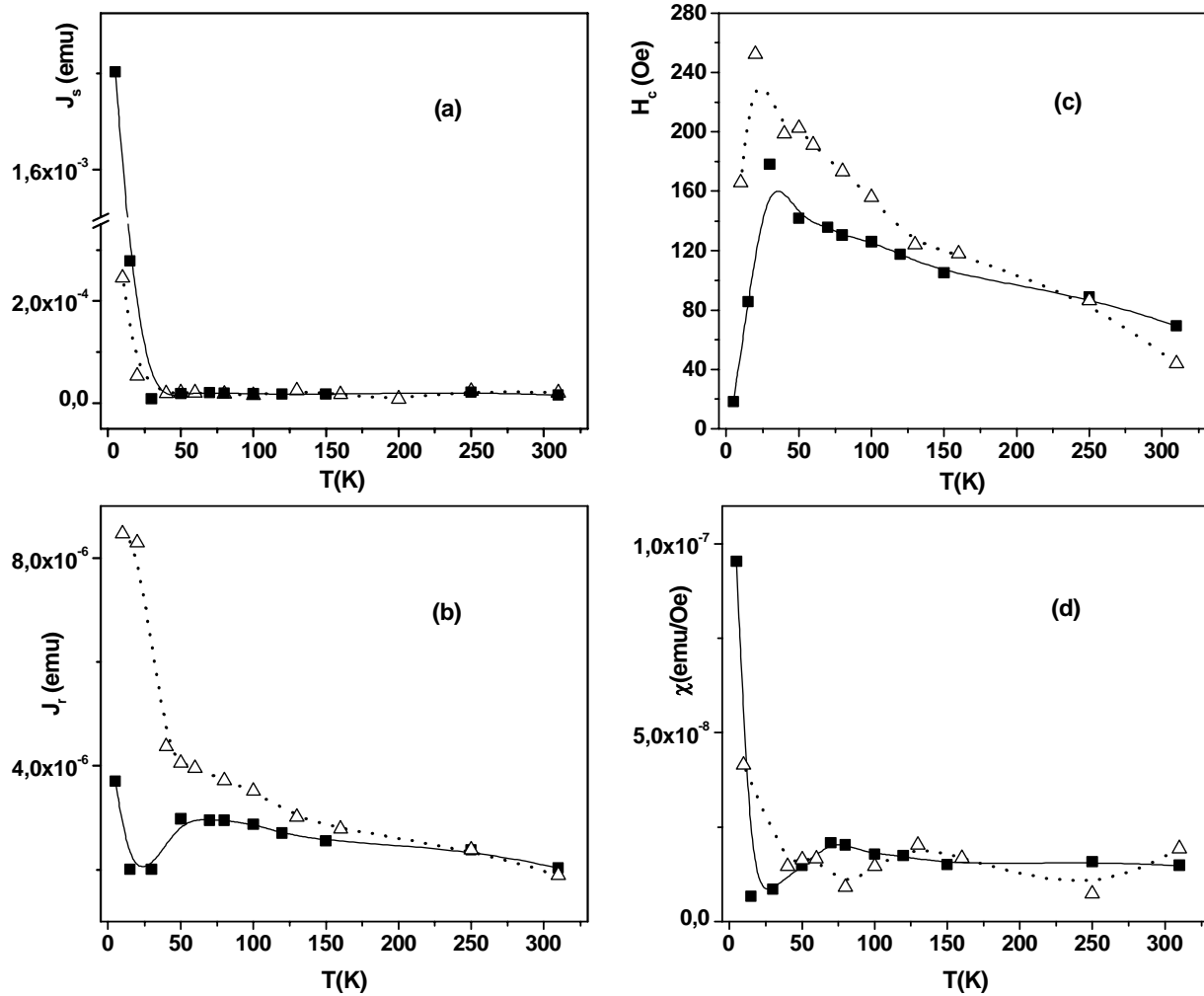
Figure 2. Temperature dependence of magnetic parameters. (a) Saturation magnetization, J_s , (b) Remanent magnetization, J_r , (c) Coercive field, H_c and (d) Initial susceptibility, \chi . Abdomen segments of eight bees oriented perpendicular (full square) and parallel (open triangle). Lines are guides to the eyes.
