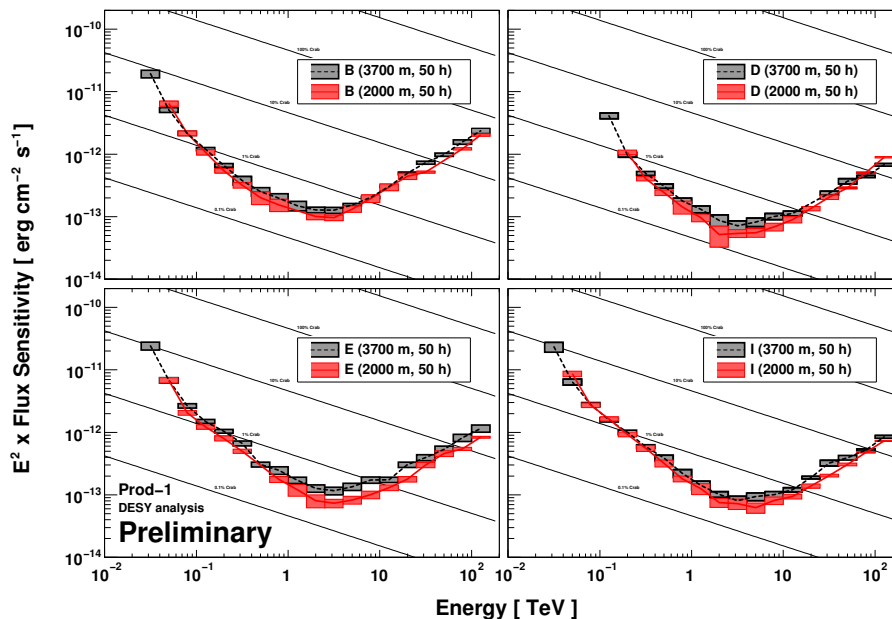
Fig. 5: Differential sensitivity of the four layout candidates from Figure 1 at 2000 m altitude (red, solid line) and 3700 m (black, dashed line), based on the DESY analysis ( 20^\circ zenith angle, 50 h observation time). Apart from the different altitude, the simulations are for the same hypothetical site configuration.
